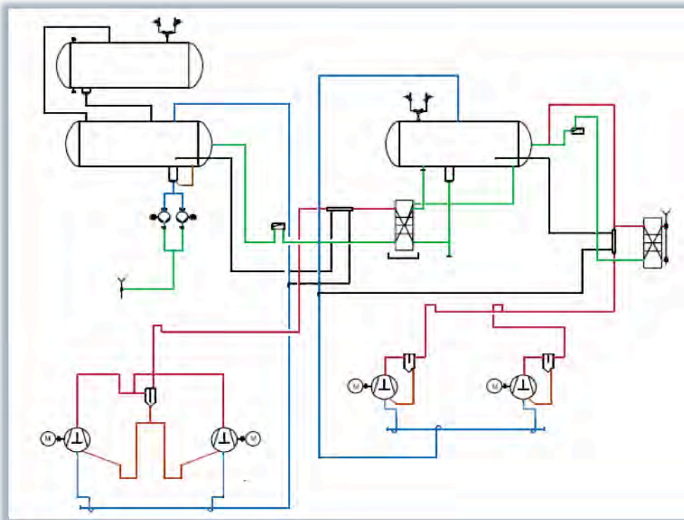
Schematic PI-diagram of the CO 2 / propene-cascade refrigeration system
